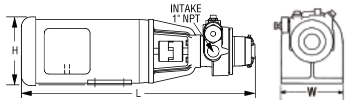
Flange Mounting – XF1 / XF1P
